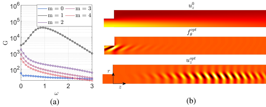
Figure 1: Linear resolvent analysis at Re = 1200 . a) Harmonic optimal gain for azimuthal numbers m \in [0, 4] . b) top: streamwise velocity of the base flow, middle and bottom: azimuthal component of the optimal forcing and response for \omega = 0.94 , m = 1 .
