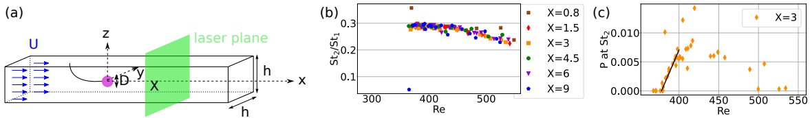
Figure 1: (a): schematic of the experimental set-up. (b) : Ratio St_2/St_1 as a function of the Reynolds number. (c) : orange diamonds : power associated to the low frequency St_2 , as a function of the Reynolds number, straight line: linear fit.
